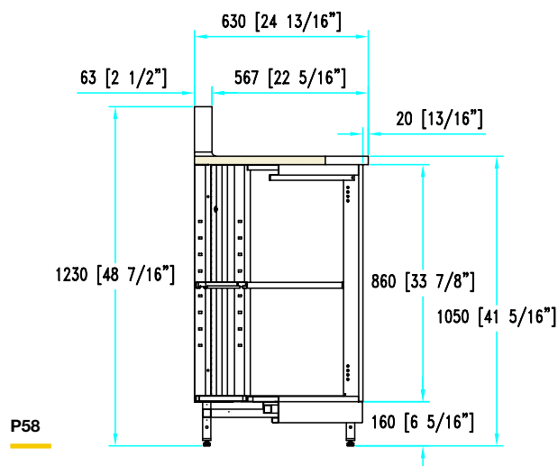
Outside corner 90° Open storage
