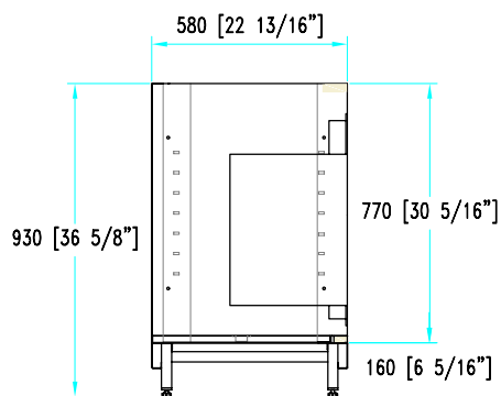
Single garbage hopper
