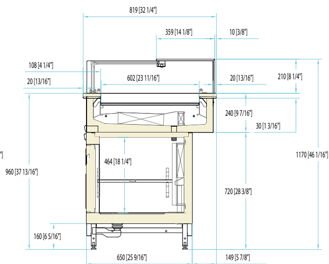
H117 Display cabinet with glued glass lighted case and refrigerated storage
