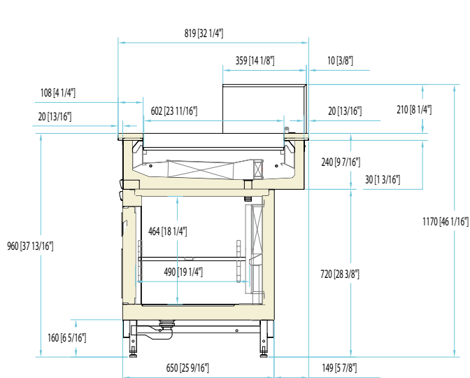
H117 Display cabinet with glued glass open case and refrigerated storage (only extra EU)
