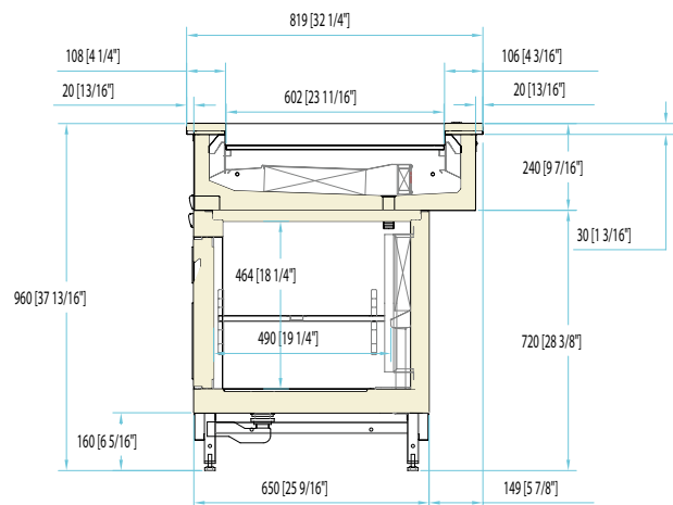
Well on refrigerated storage counter base
