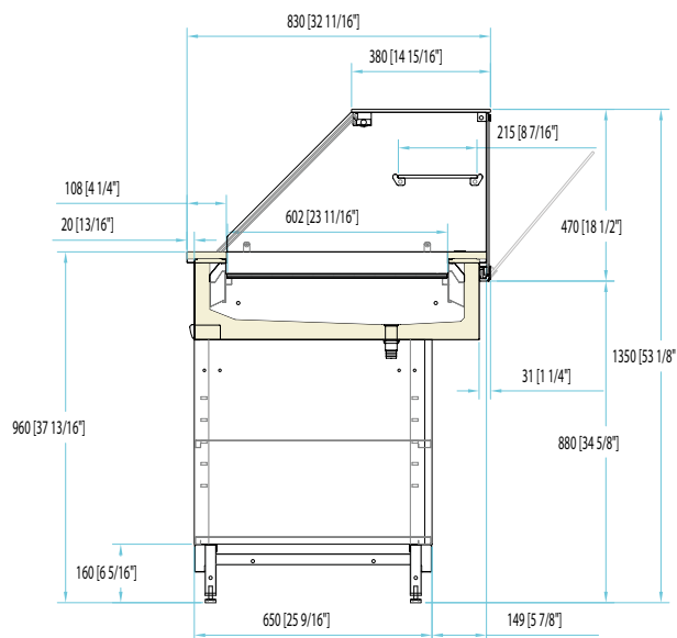
H135 Display cabinet with lighted tilt glass structure on neutral counter base
