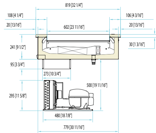
Well with factory-connected condensing unit
