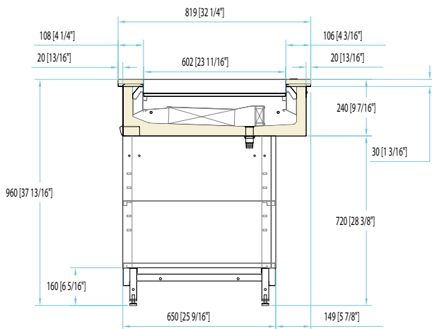
Well on neutral counter
