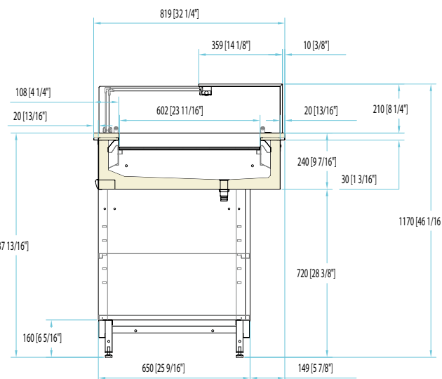
H117 Display cabinet with glued glass lighted case on neutral counter base
