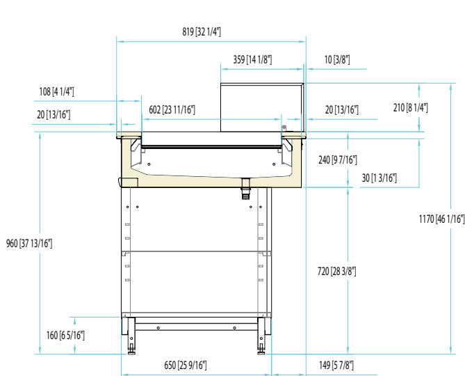
H117 Display cabinet with glued glass open case on neutral counter base
