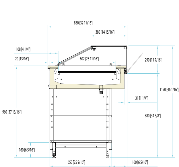
H117 Display cabinet with lighted tilt glass structure on neutral counter base
