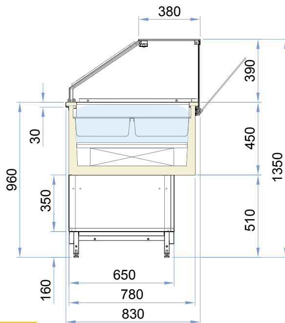
H135 Tilt glass with LED lighting and sliding doors
