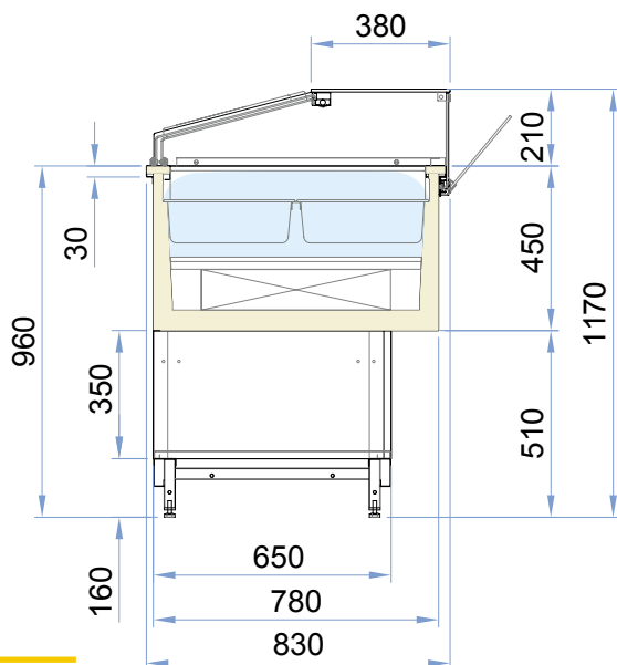
H117 Tilt glass with LED lighting and sliding doors
